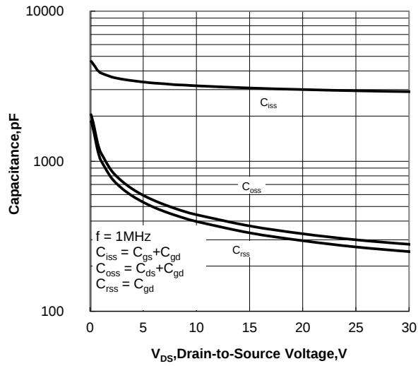
Figure 12. Capacitance Characteristics
