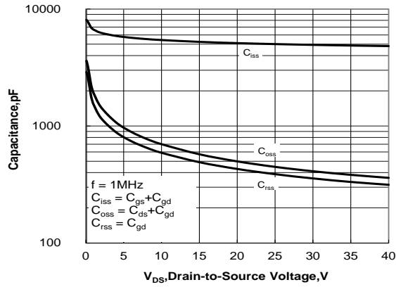
Figure 12. Capacitance Characteristics
