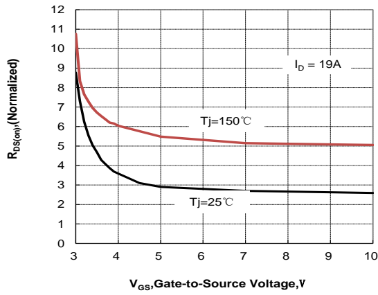
Figure 14. Normalized On Resistance vs VGS
