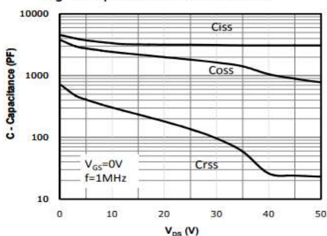
Fig 6: Capacitance Characteristics
