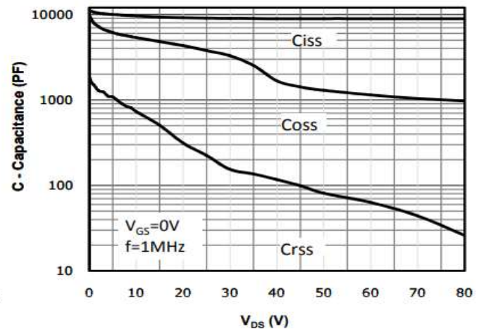
Fig 6: Capacitance Characteristics
