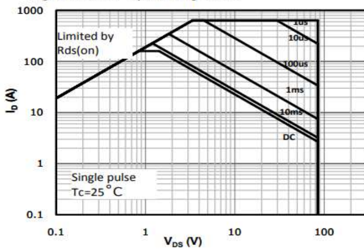
Fig 11: Safe Operating Area
