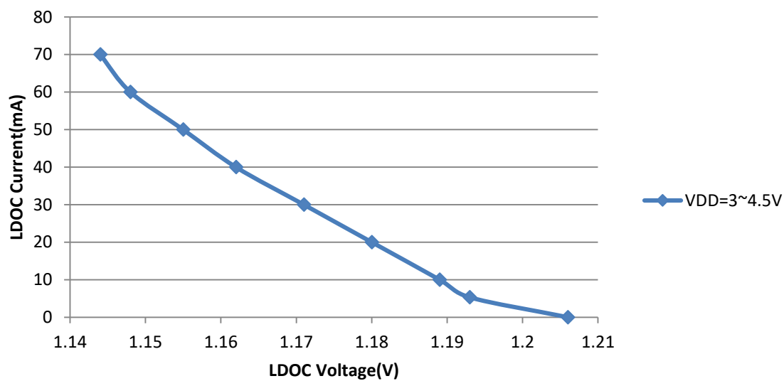
LDO Current vs. Voltage
