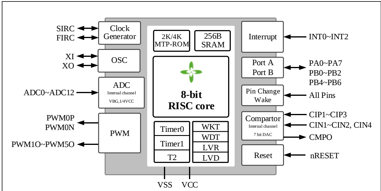
TM56M1522/22B/22C/21H Block Diagram
