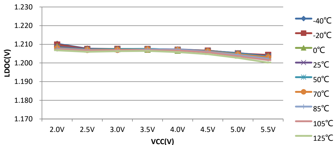
LDO Voltage vs. VCC
