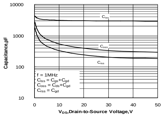
Figure 12. Capacitance Characteristics
