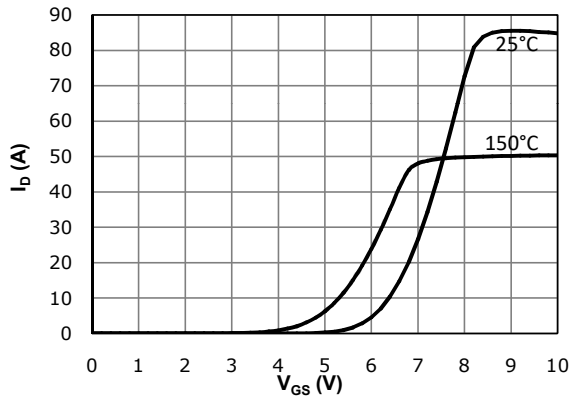
Fig 3: Transfer Characteristics
