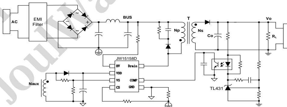
JW15158D Typical Application
